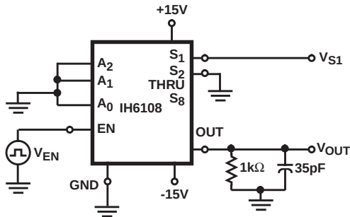
FIGURE 3. t_{\text{ON}} AND t_{\text{OFF}} SWITCHING TEST CIRCUIT AND WAVEFORMS
